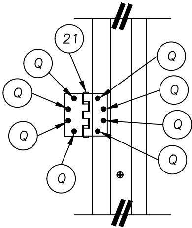
HINGE DETAIL
